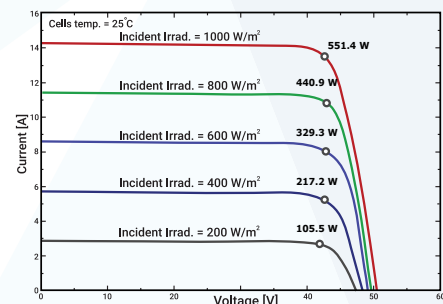
I-V Curve of 550W at 25°C cell temp. and different Irradiance level
