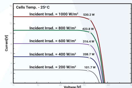
I-V Curve of 530W at 25°C cell temp. and different irradiance level
