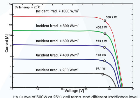
I-V Curve of 500W at 25°C cell temp. and different Irradiance level
