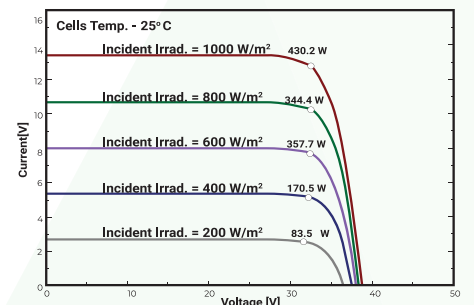
I-V Curve of 430W at 25°C cell temp and different Irradiance level
