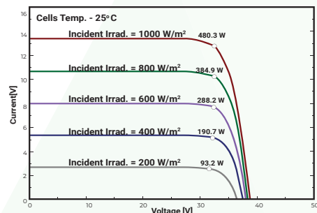
I-V Curve of 480 W at 25°C cell temp and different Irradiance level
