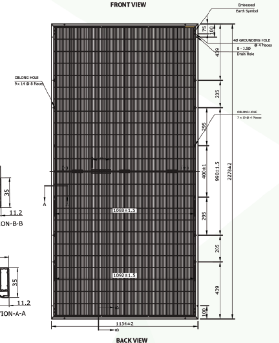
BACK VIEW
