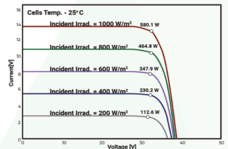
I-V Curve of 580W at 25°C cell temp. and different Irradiance level
