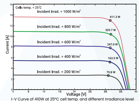
I-V Curve of 410W at 25°C cell temp. and different irradiance level
